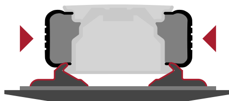
External Rim Clamping
