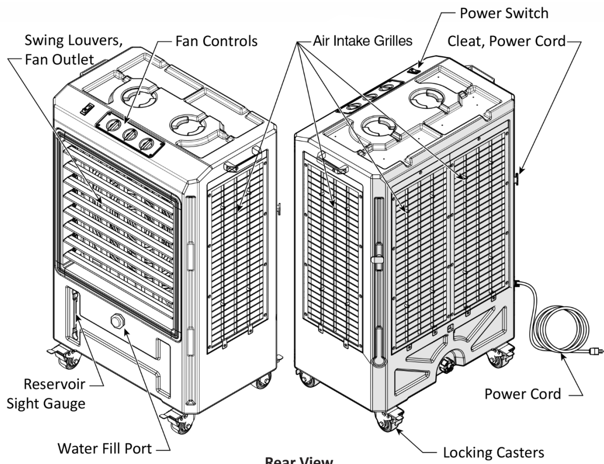
Rear View Cooling Media and retainers removed for clarity.
