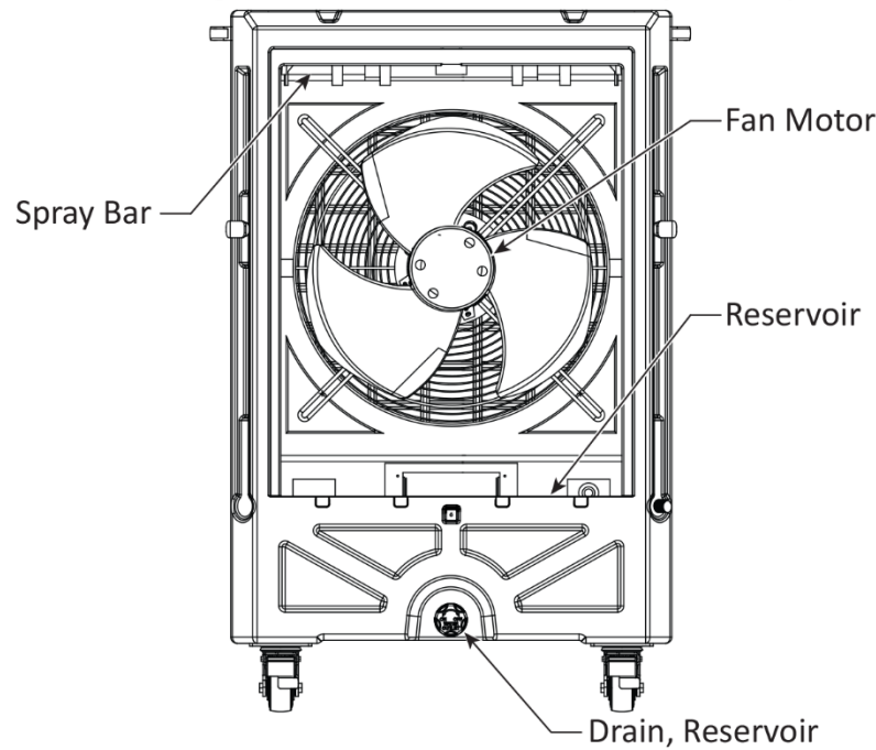
Rear View Cooling Media and retainers removed for clarity.
